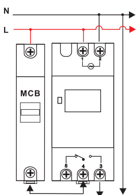
TM-919s(5P)16A
